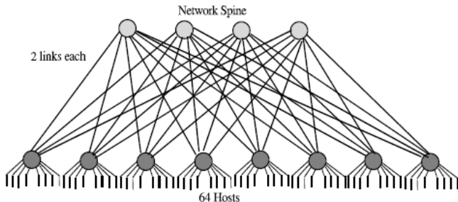
Figure: A 64-host Clos network using 16-port Myrinet switch (each line represents two links).
