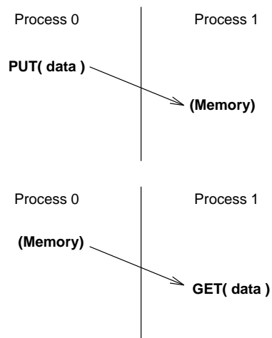
Figure 2: One sided-Communicating with other processes.
