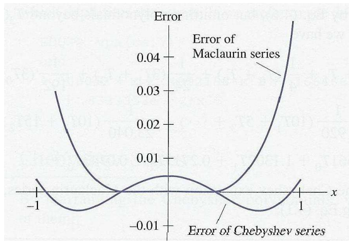
Figure: Comparison of the error of Chebyshev series for e^x with the error of Maclaurin series.
