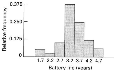
Figure: Relative frequency histogram.
