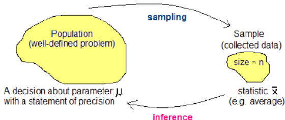
Figure: The Cycle of Statistical Procedure.
