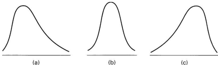
Figure: Skewness of data.
