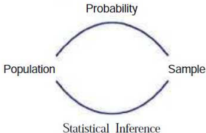
Figure: Fundamental relationship between probability and inferential
