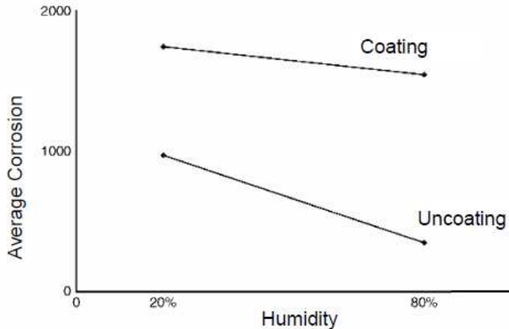
Figure: Corrosion results for Example 1.3.
