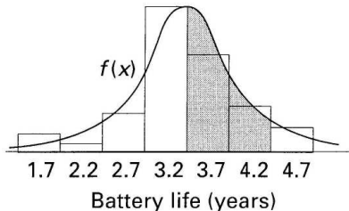
Figure: Estimating frequency distribution.
