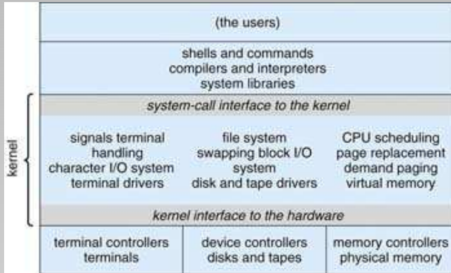
Figure: UNIX system structure.
